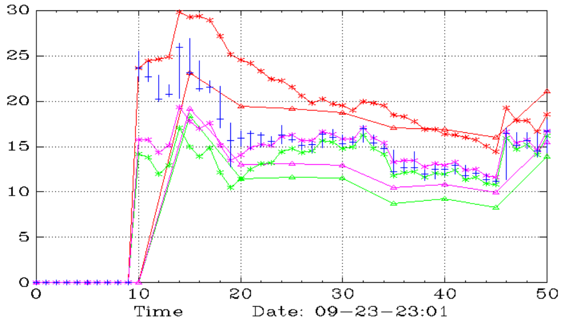
XRP (Monthly,Weekly)
