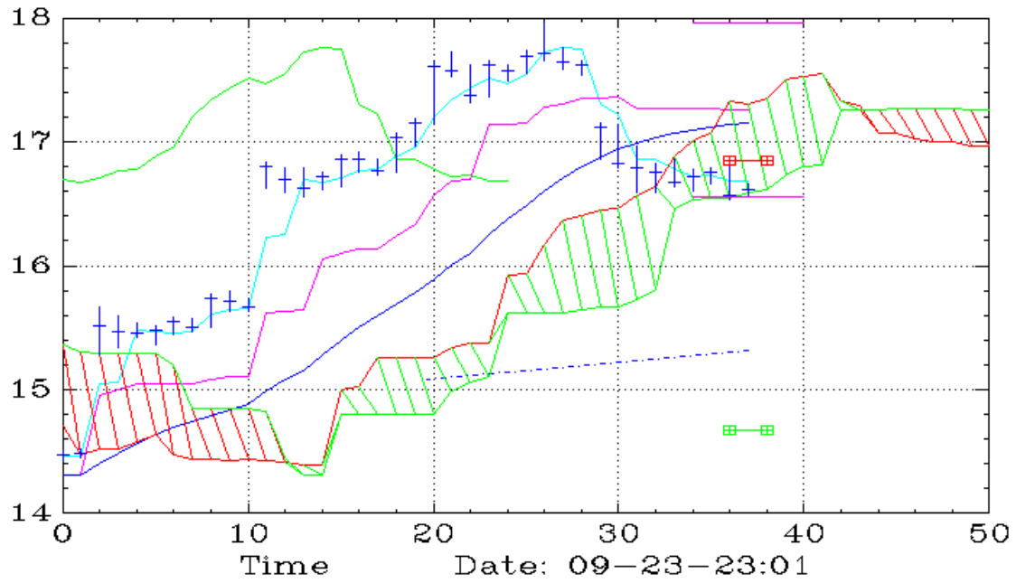
XRP (45,Ichimoku)
