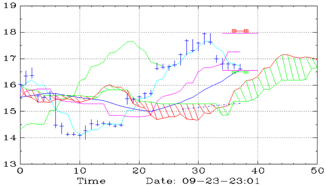
XRP (90,Ichimoku)
