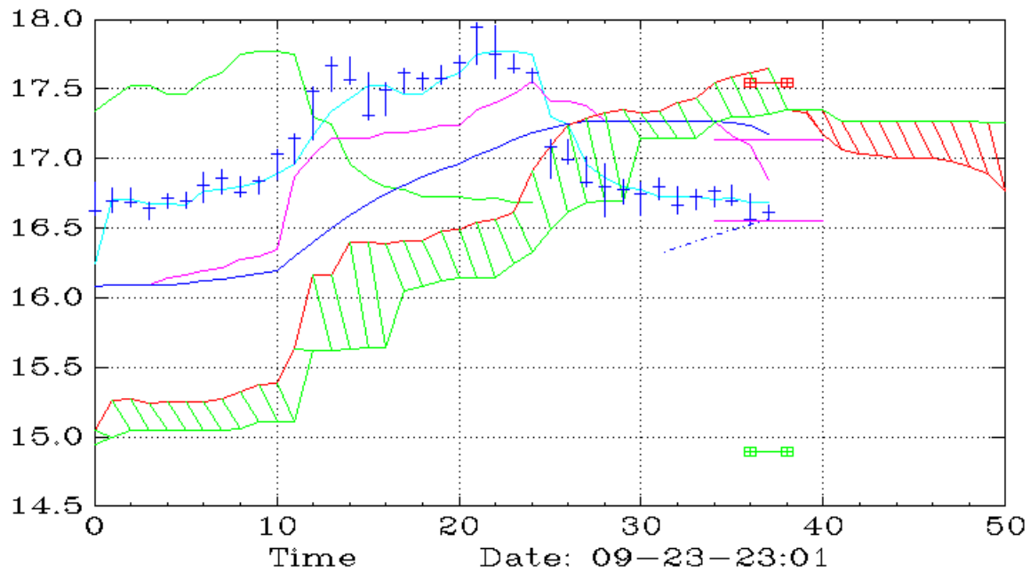
XRP (30,Ichimoku)
