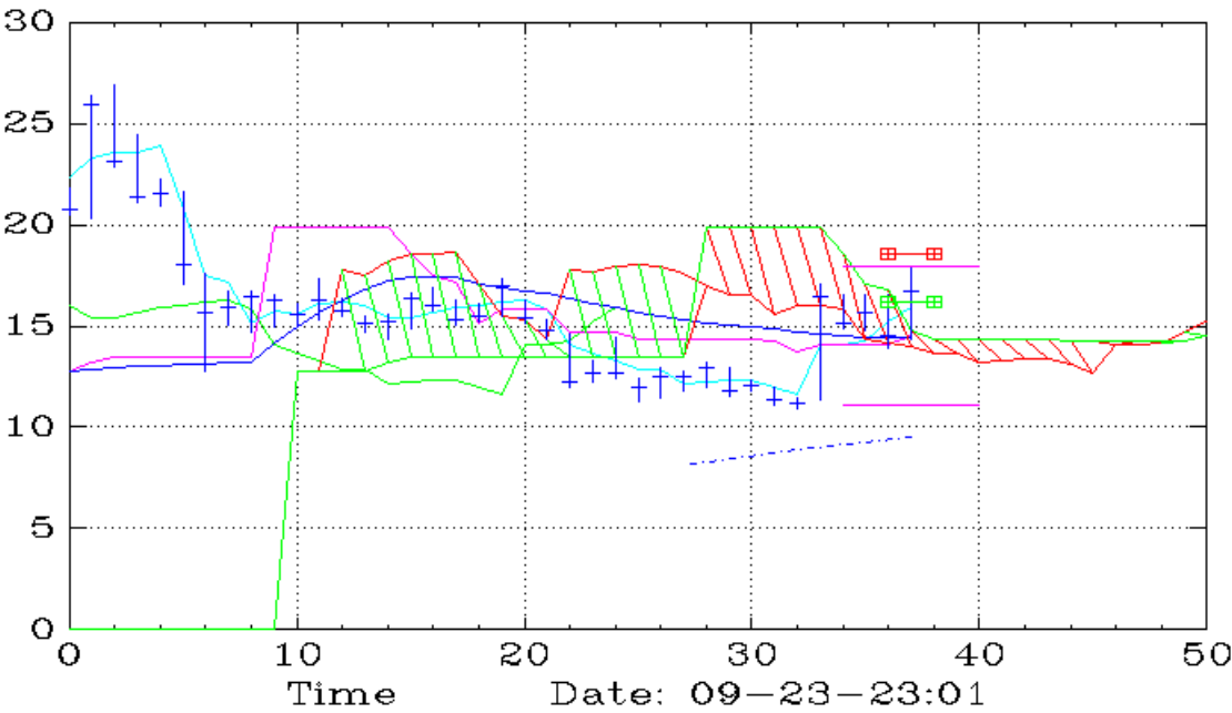
XRP (Weekly,Ichimoku)
