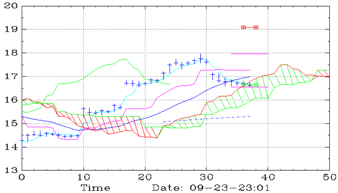
XRP (60,Ichimoku)
