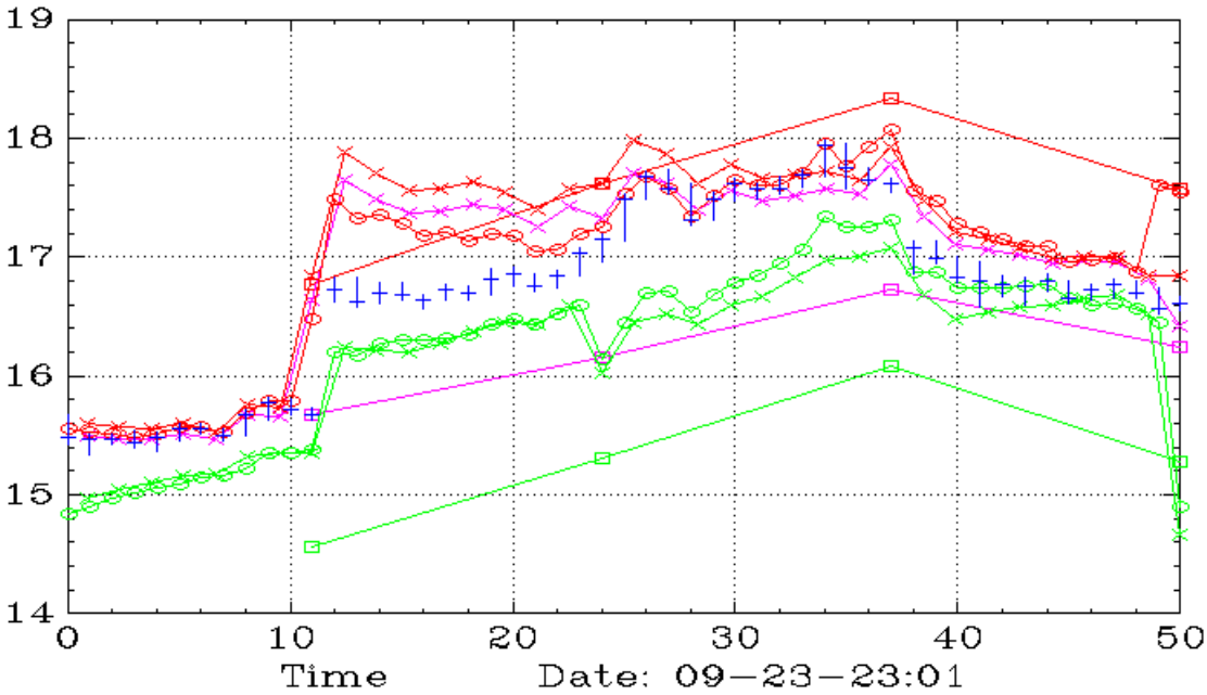
XRP (Daily,45,30)
