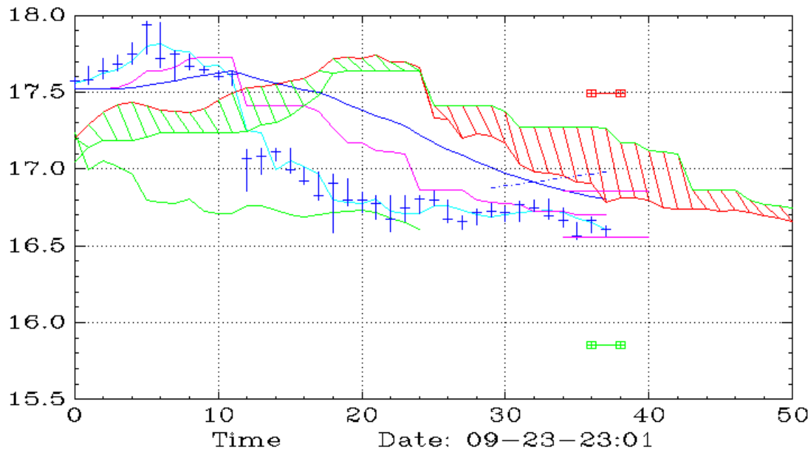
XRP (15,Ichimoku)
