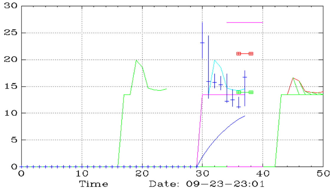
XRP (Monthly,Ichimoku)
