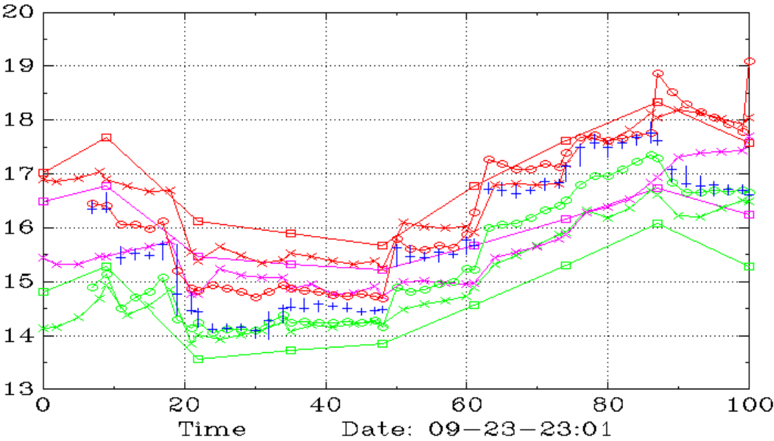
XRP (Daily,90,60)
